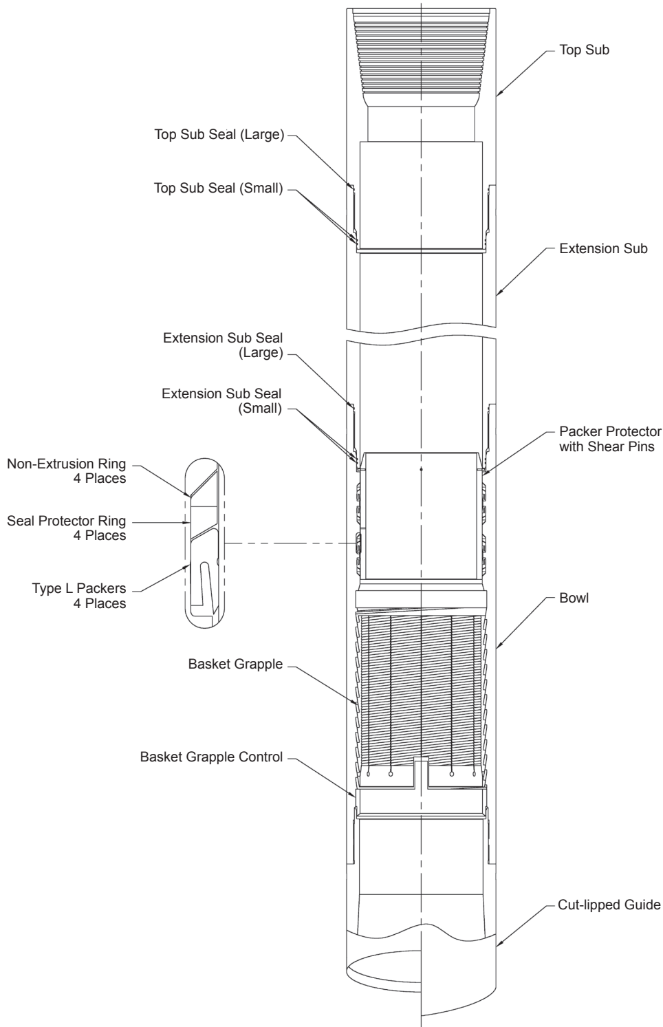
Type L Packer Type Casing Patch 15K Assembly
